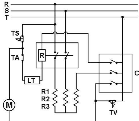
ELECTRICAL DIAGRAM 5/9kW
