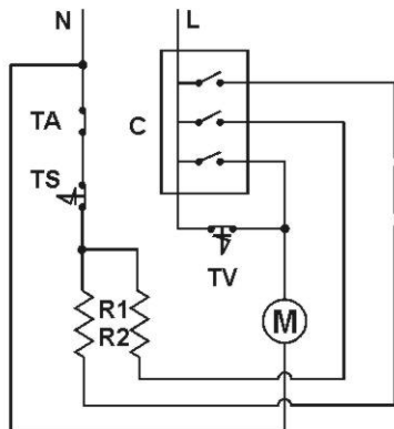
ELECTRICAL DIAGRAM 2/3/3,3kW
