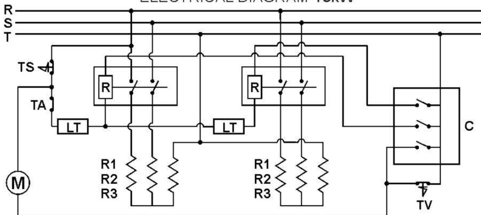
ELECTRICAL DIAGRAM 15kW
