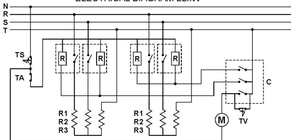
ELECTRICAL DIAGRAM 22kW
