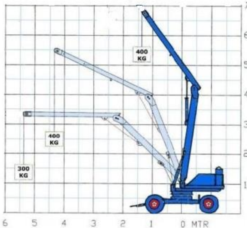
WARRY ELEMENTENSTELROBOT BY400.P/UG
