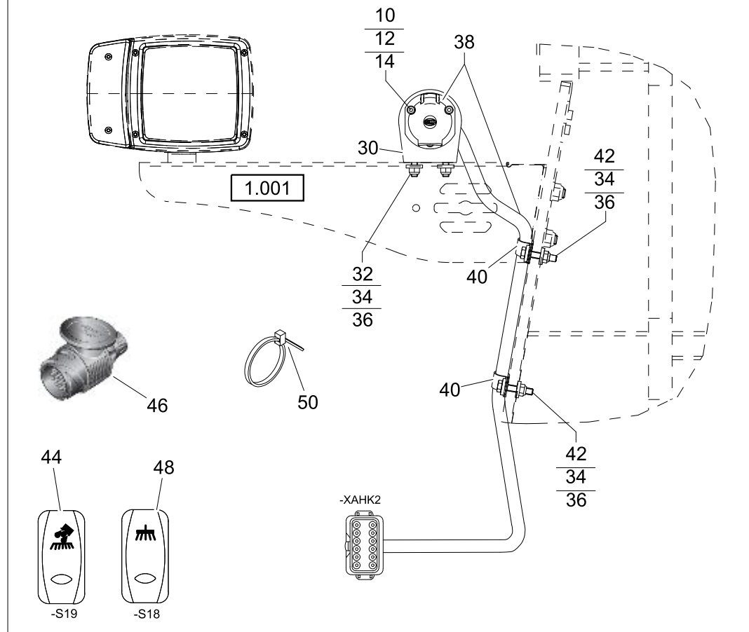
Steckdose am Lampenhalter 13-Polig 13-pin socket at the lamp holders.
