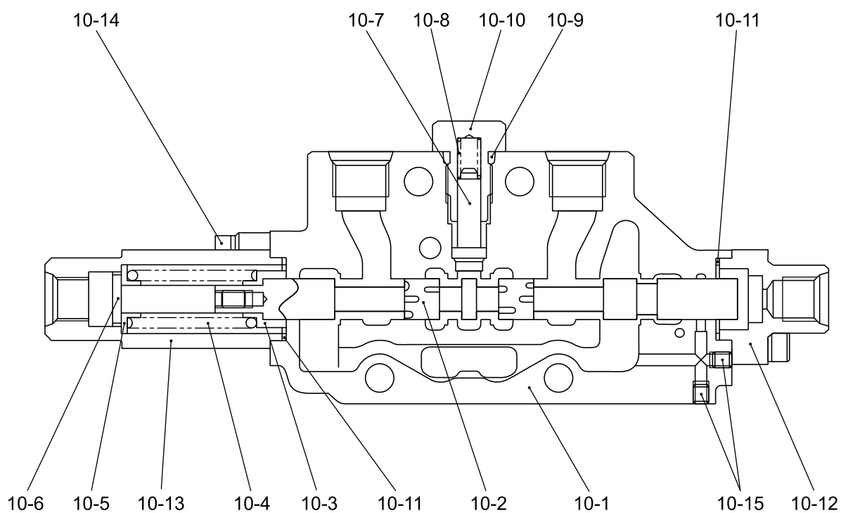
SECTION J-J
