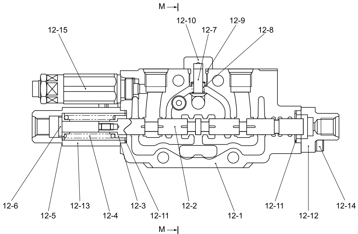
SECTION L-L
