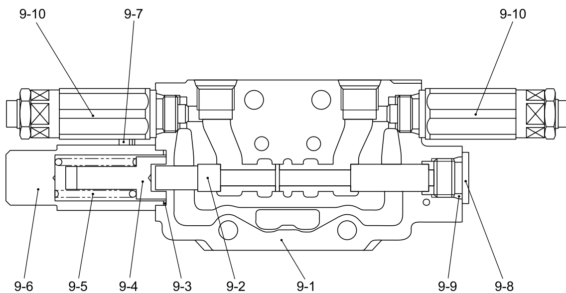
SECTION I-I
