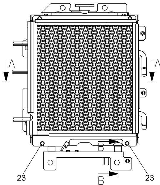
矢視 I VIEW I
