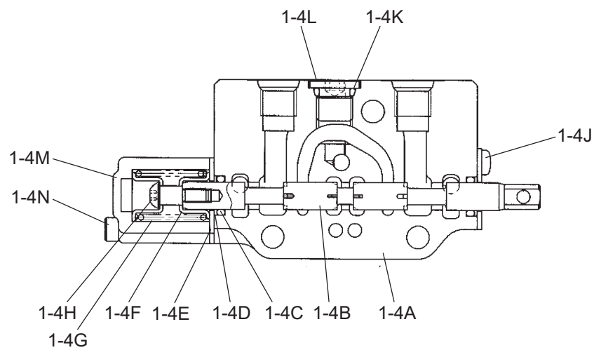
D-D H-H (走行・TRAVEL)
