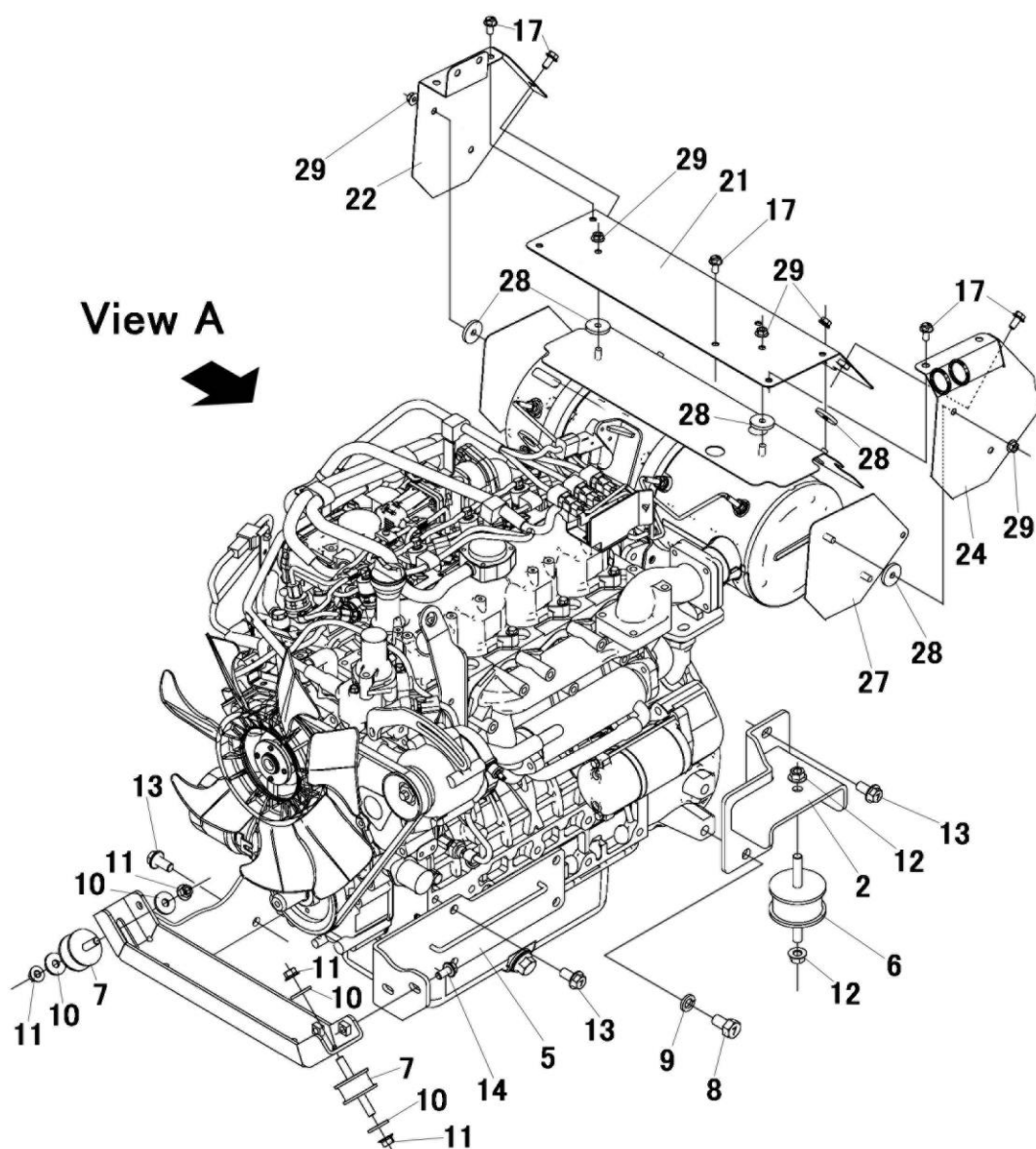
View A (ENGINE LEFT SIDE)
