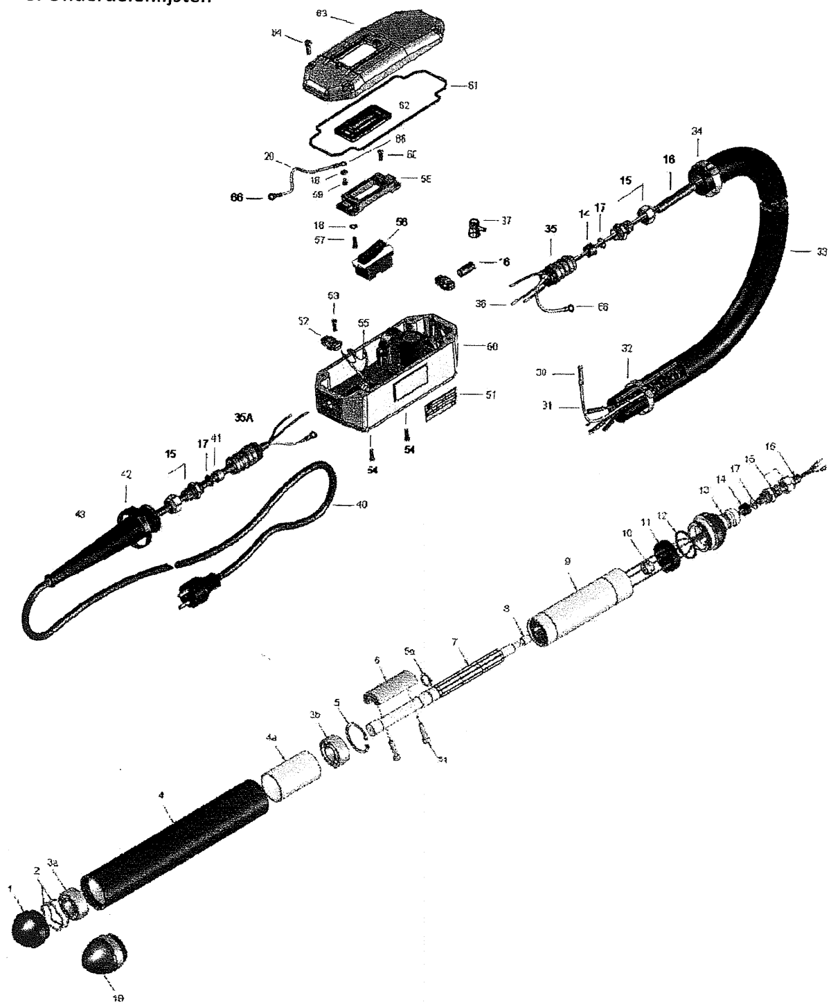
Figuur 3: Exploded view LHF-E
